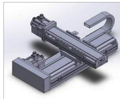
FTH17-FTH14-XY-S
